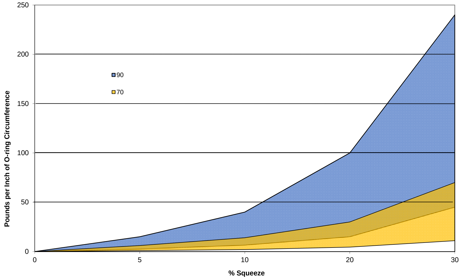
Compressive Load Force, 90 & 70 duro, 0.139" CS
