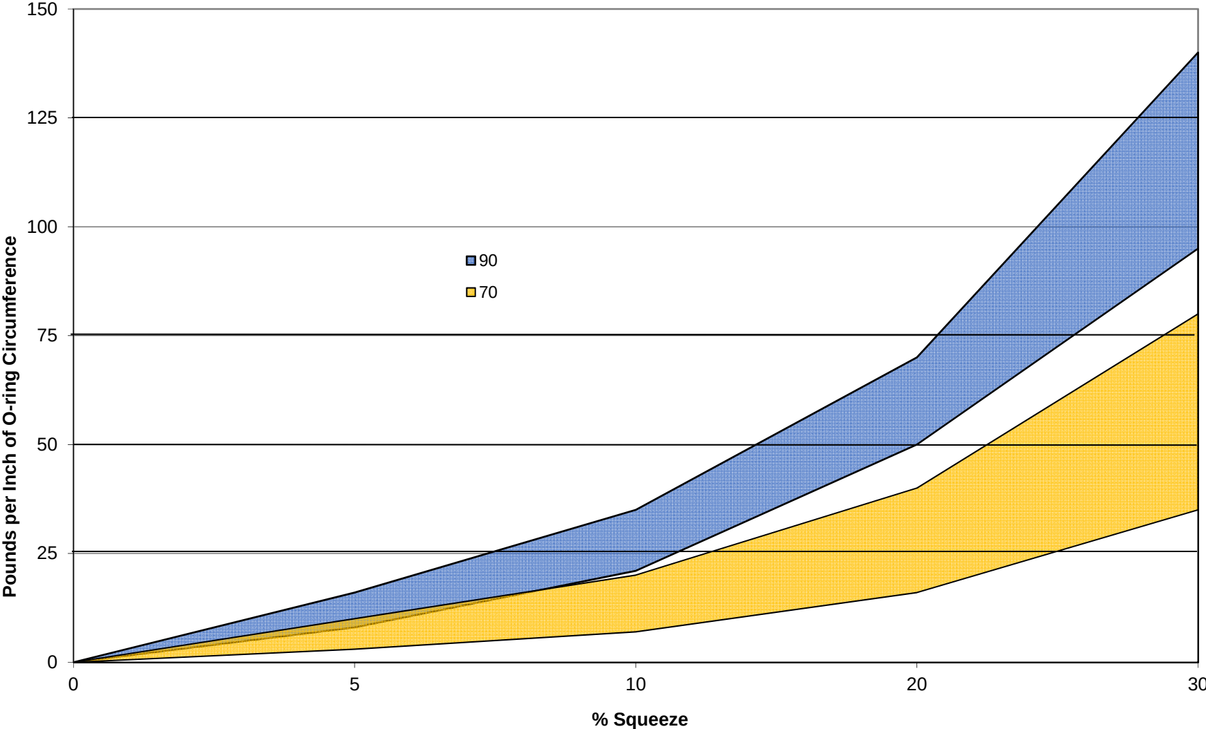
Compressive Load Force, 70 & 90 duro, 0.210" CS
