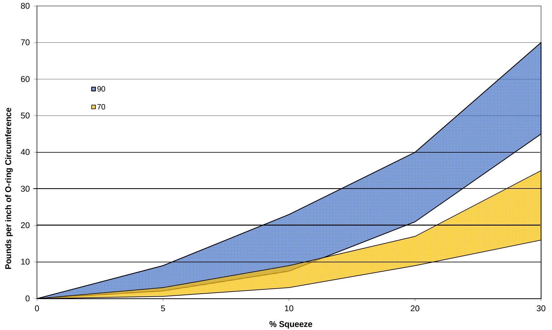
Compressive Load Force 90 & 70 duro, 0.103" CS
