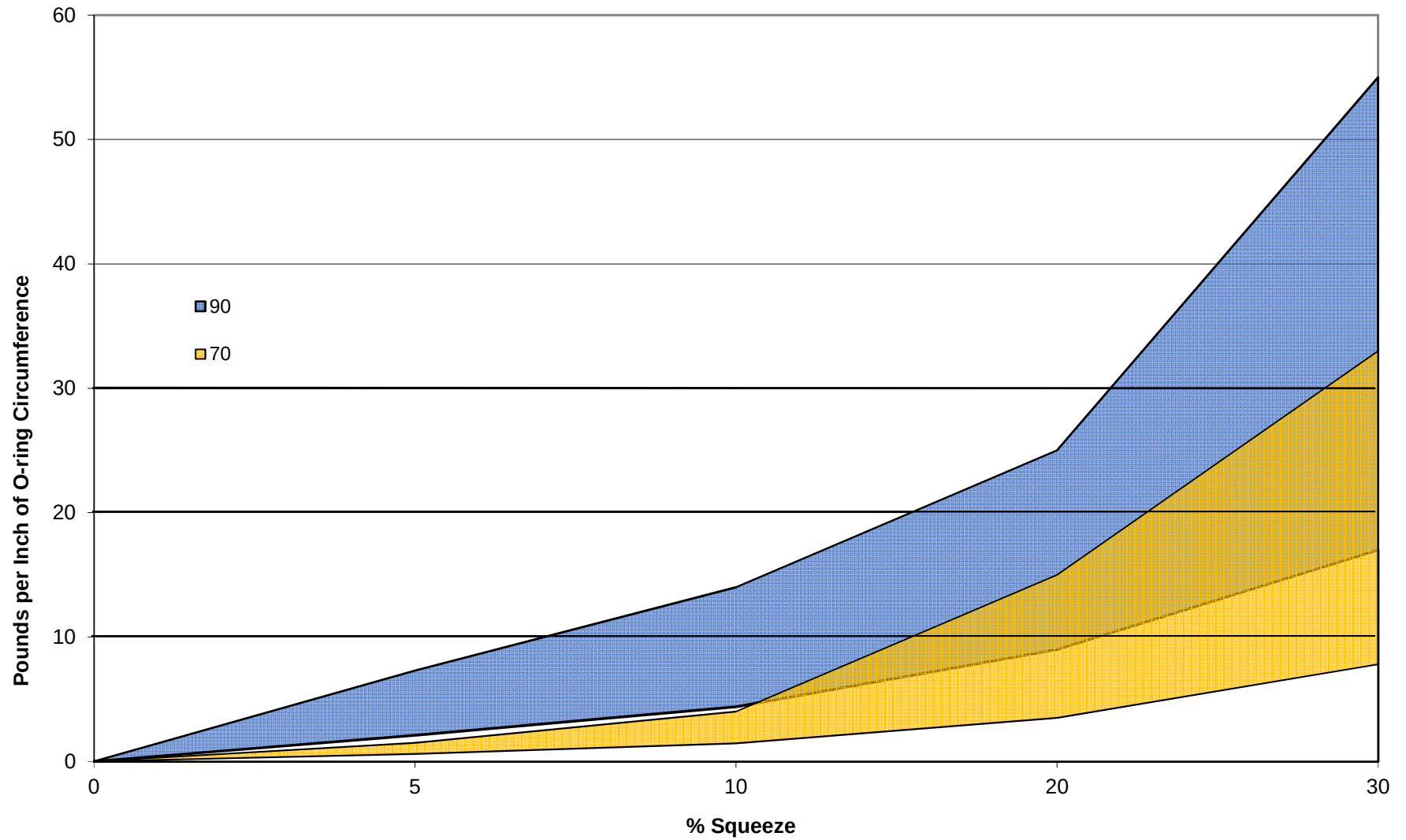
Compressive Load Force, 70 & 90 duro .070"
