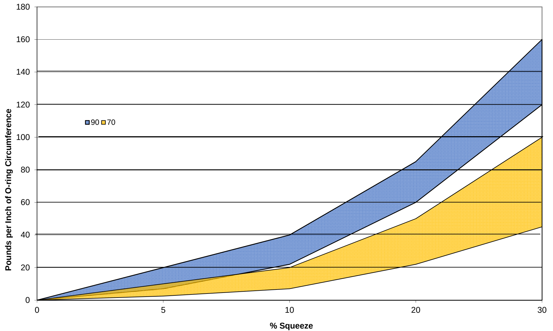
Compressive Load Force, 70 & 90 duro, 0.275" CS
